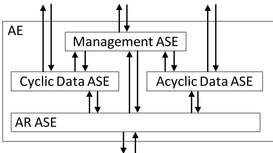
Figure 4 – Structure of ASE type S of FAL type 25
