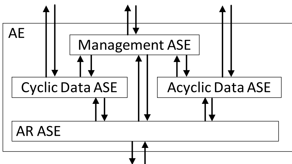
Figure 5 – Structure of ASE type N of FAL type 25
